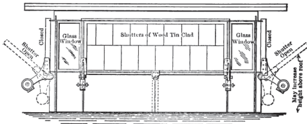
SMOKE VENT. MONITOR TYPE SIDE ELEVATION
