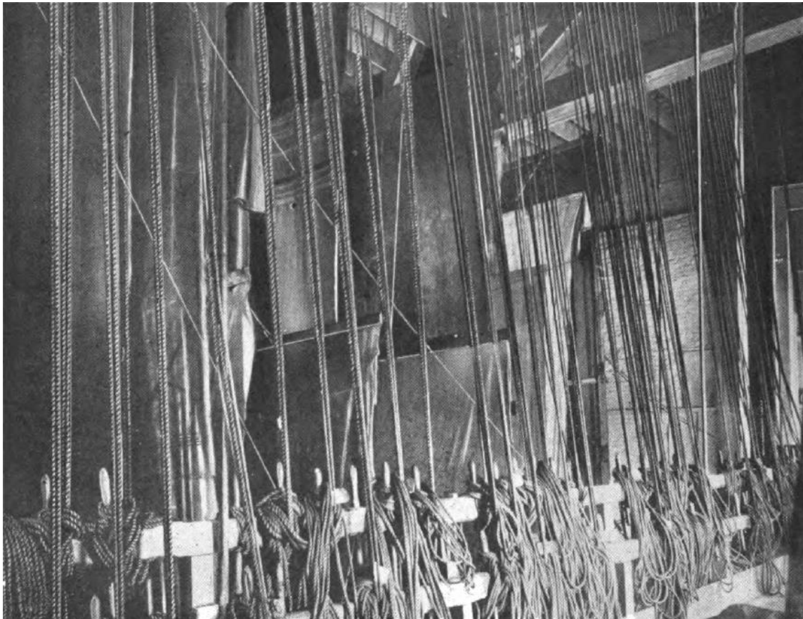
Fig. 1. — Typical view over a theater stage, above the level of the proscenium arch, showing the canvas scenery, the ropes by which it is raised and lowered, and the "pin-rail" on which these ropes are fastened.
