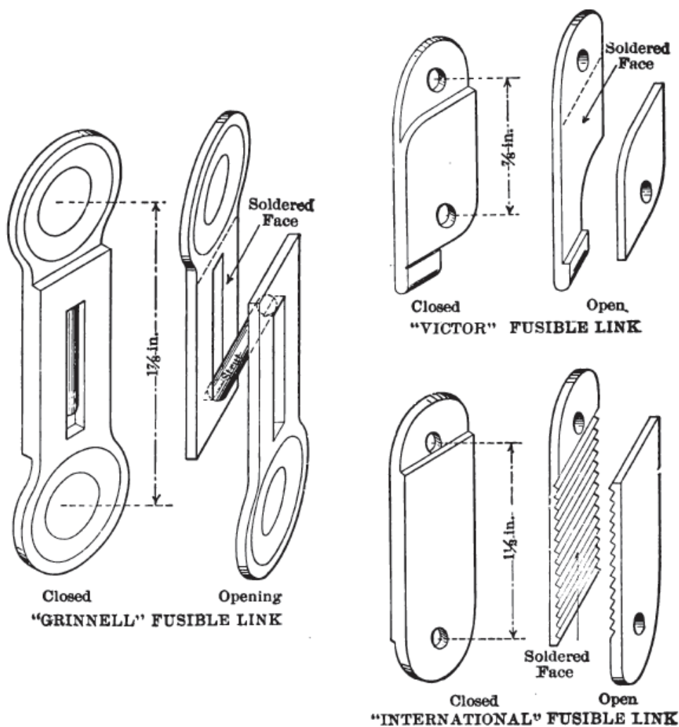
Fig. 4. — Fusible Links for Fire Protection.
