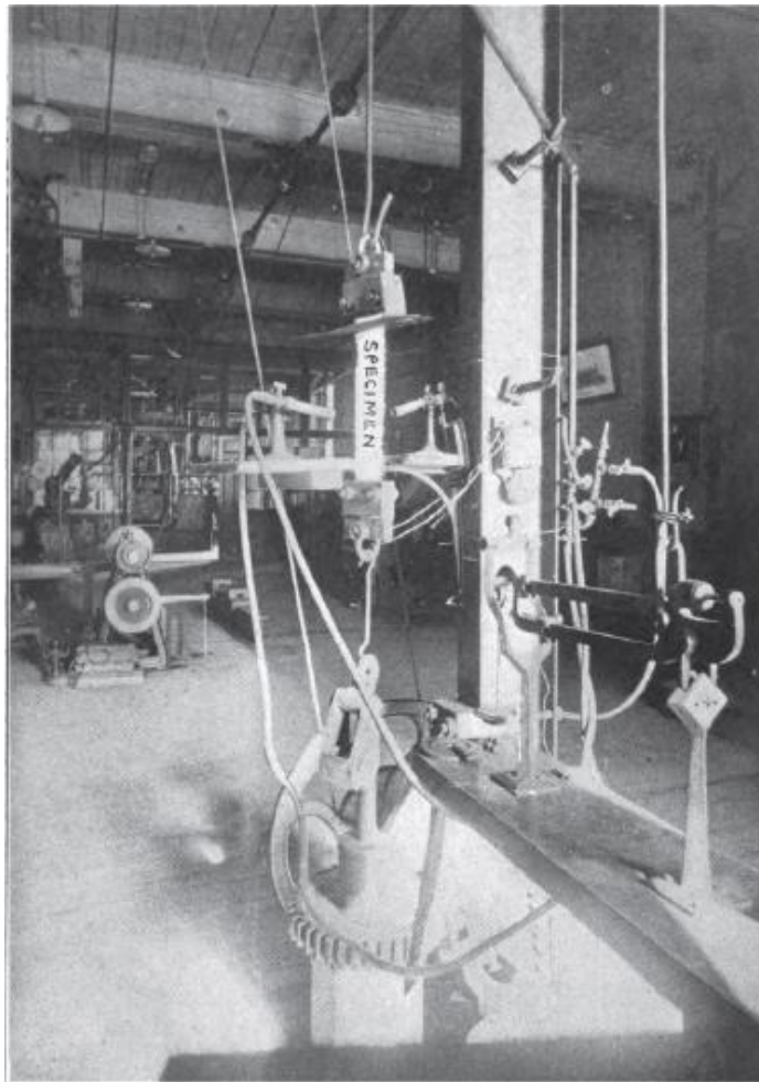
Fig. 9.— Arrangement for tests of strength of asbestos canvas in mechanical engineering laboratory, Massachusetts Institute of Technology. Tensile strength measured either cold or while heated by common gas flame or by blast lamp flame to various degrees.
