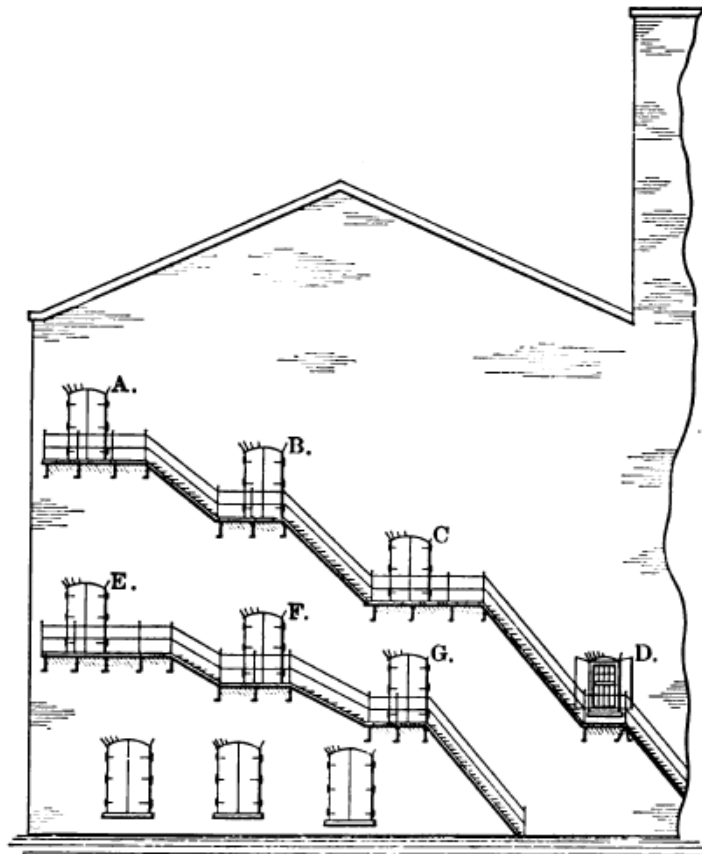
Fig. 14.—Emergency Exits in Rear of Iroquois Theater.
