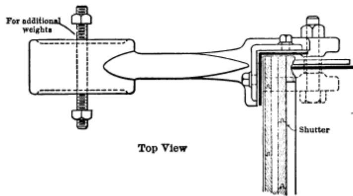
DETAIL OF WEIGHT FOR SHUTTER OF SMOKE VENT, MONITOR TYPE FIG. 5D.
