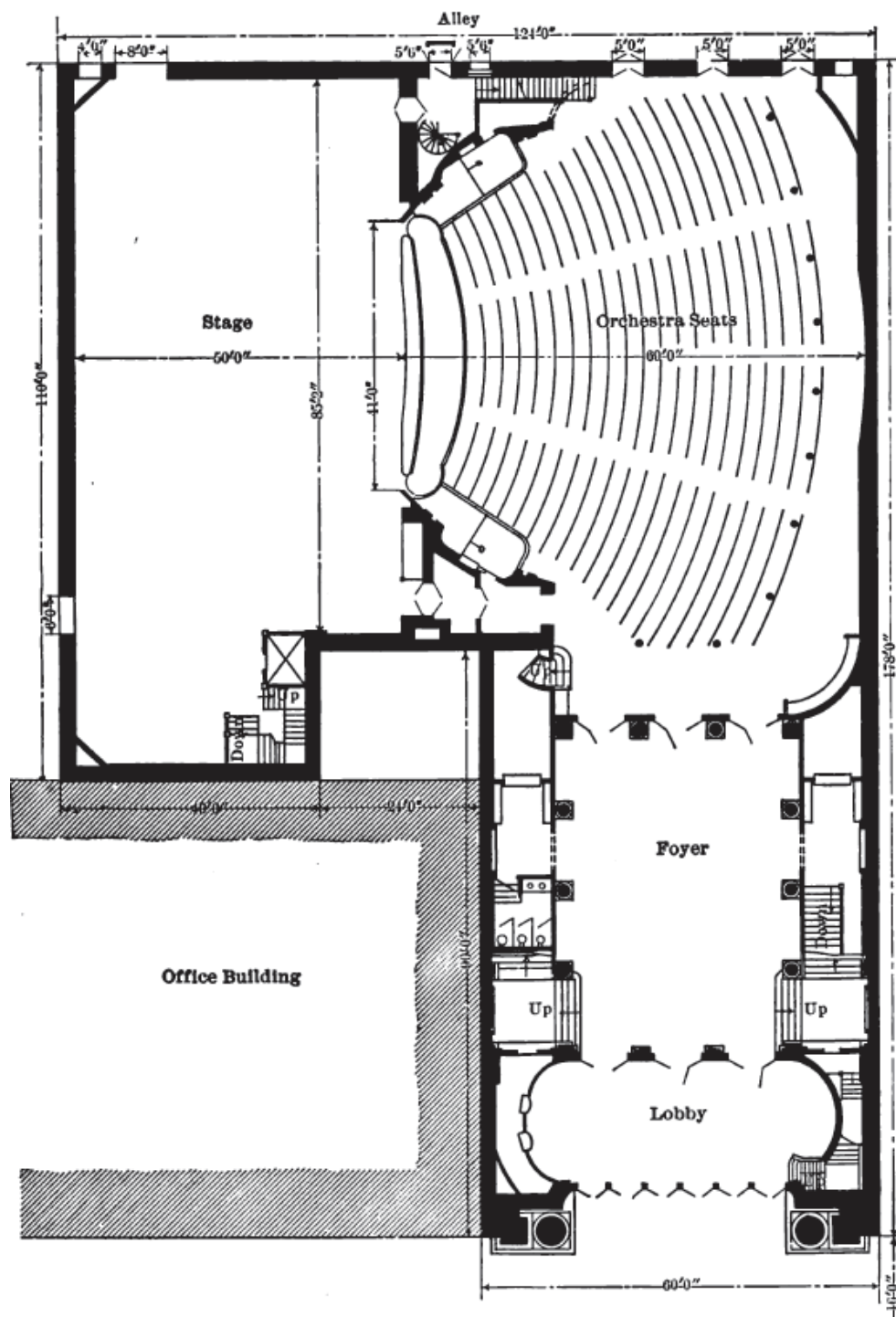
Fig. 3a.— Ground plan of Iroquois Theater, facing Randolph St.
