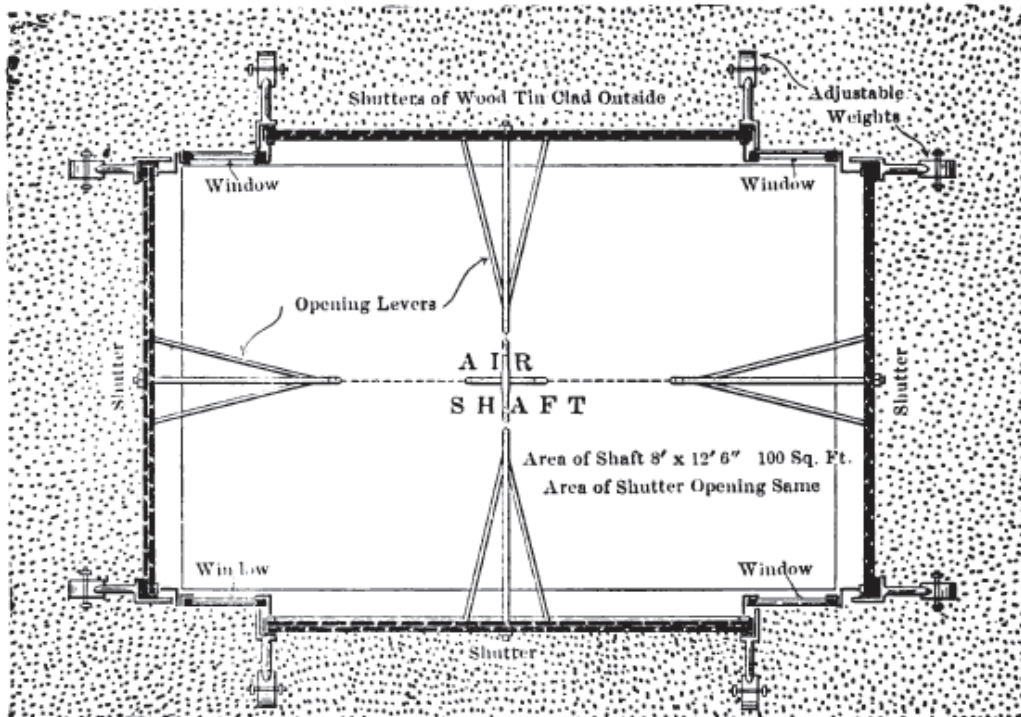
SMOKE VENT. MONITOR TYPE HORIZONTAL SECTION
