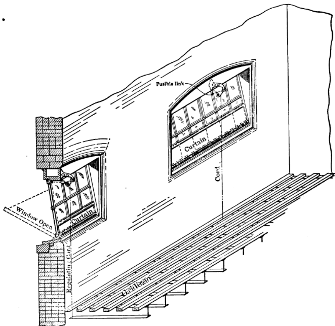
FIG. 7.—AUXILIARY SMOKE VENTS IN WALL ABOVE GRIDIRON.
