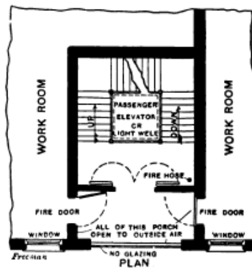
FIG. 16.—TOWER FIRE ESCAPE FOR FACTORIES. PHILADELPHIA TYPE.
